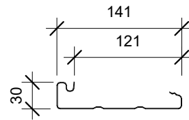
136 FASCIA COVER = 121mm
