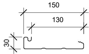
150 FASCIA COVER = 130mm
