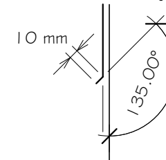
KICK-OUT at bottom edge of vertical flashing
