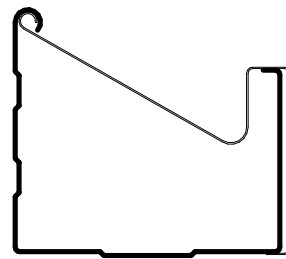
ROOFING INDUSTRIES 175 BOX GUTTER
