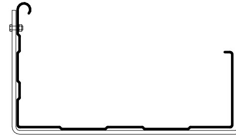
ROOFING INDUSTRIES 300 BOX GUTTER
