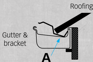
Diagram 1 - Position Leg "A" of the Ezi-Lok™ Gutter Screen into the gutter/spouting and up under the roof.
