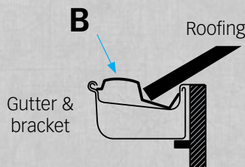
Diagram 2 - Compress the Ezi-Lok™ Gutter Screen slightly and push down the Ezi-Lok™ Gutter Screen edge "B" into the spouting/gutter beak.
