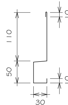
FLASHING OPTION 02
