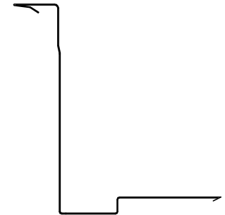
ROOFING INDUSTRIES SPANLOK™ EXTERNAL CORNER
