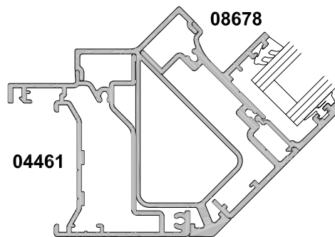
04443 135° COUPLING BAR
