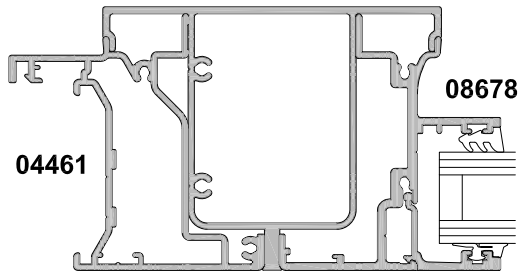
04440 180° COUPLING BAR
