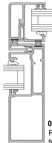
SECTION B-B
