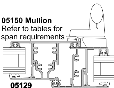
D/G Beaded Sash
