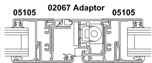
FRENCH CASEMENT WINDOW STILE OPTION
