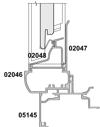
TIMBER BLADES NON-STANDARD JAMB HEIGHT
