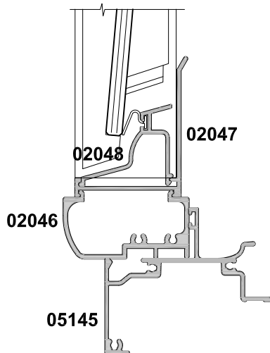
GLASS, ALUMINIUM & TIMBER BLADES STANDARD JAMB HEIGHT
