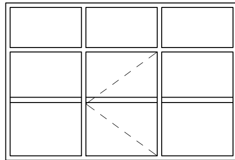
Hinged Door into 100mm Flushglaze
