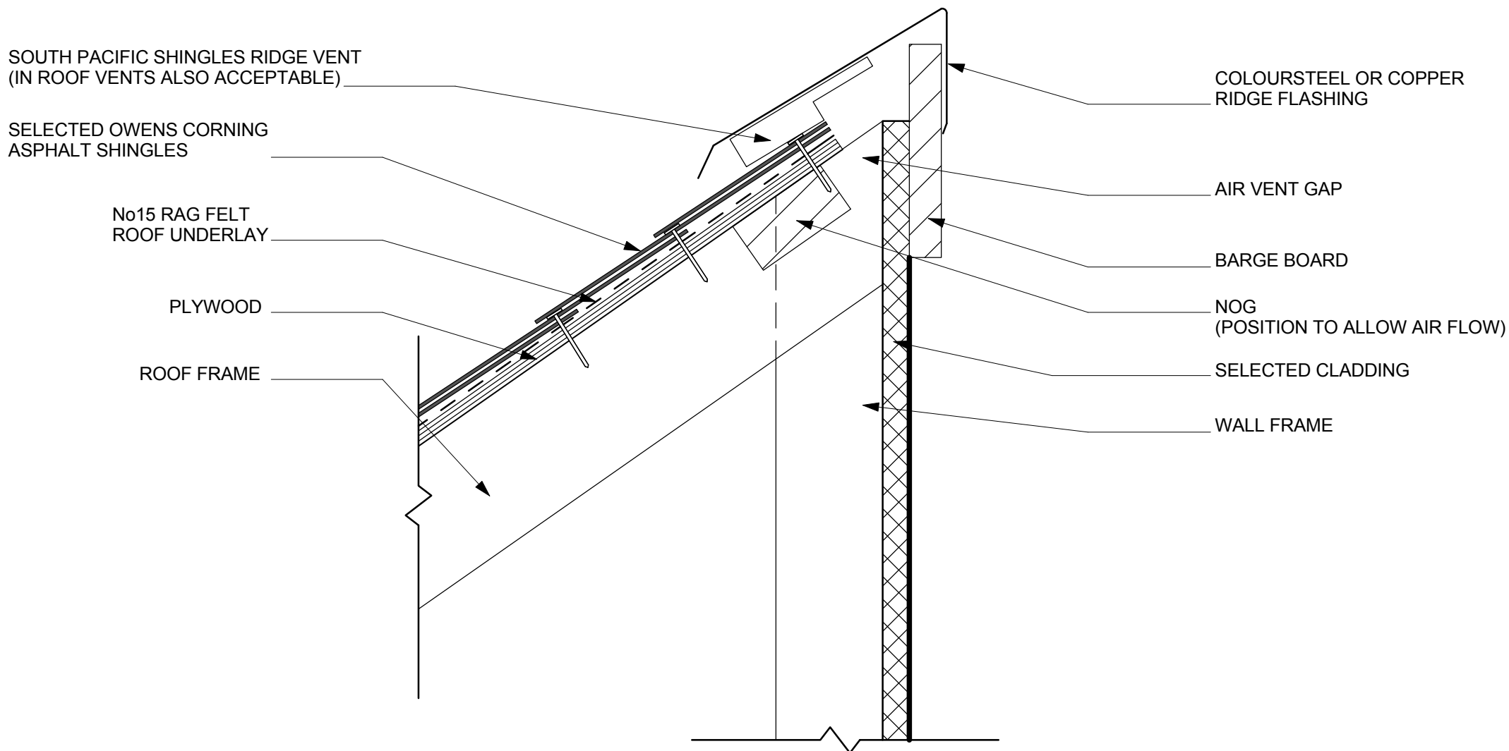
TYPICAL ROOF/WALL RIDGE DETAIL - CROSS SECTION
