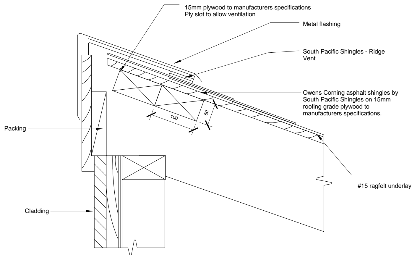
Typical Owens Corning Vented Roof to Peak
