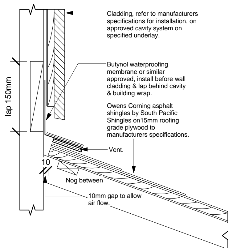
Typical Owens Corning Shingle Vented Apron Flashing - Roof to Wall
