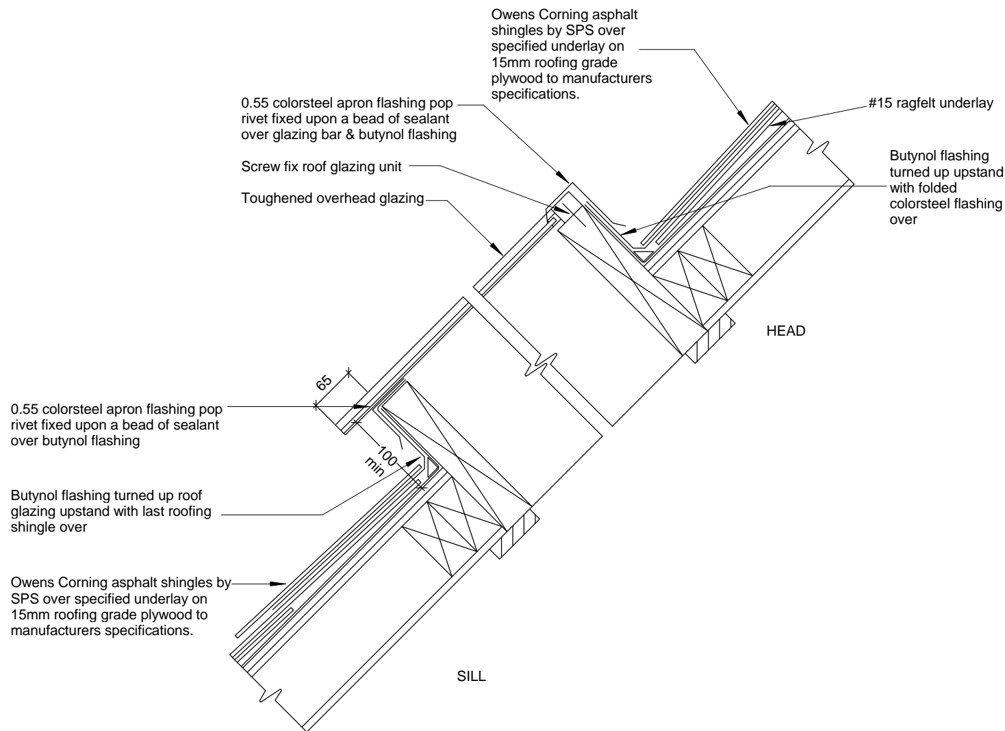
Owens Corning roof to skylight head and sill detail
