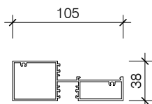
PAS021/A 105 GLAZING SILL/TRANSOM
