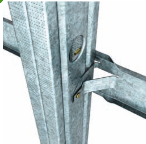
■ BACK VIEW OF FAST-FIX NOGGING®
