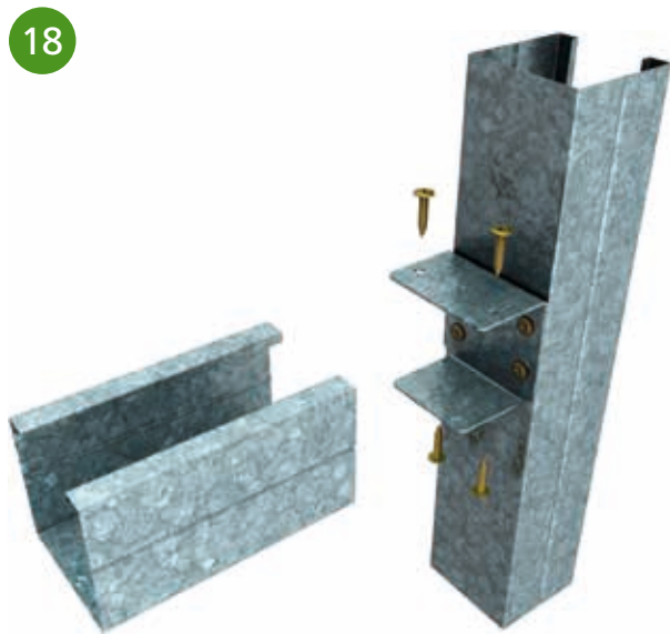
■ INSTALLATION OF DUPLEX HEADER STUD
