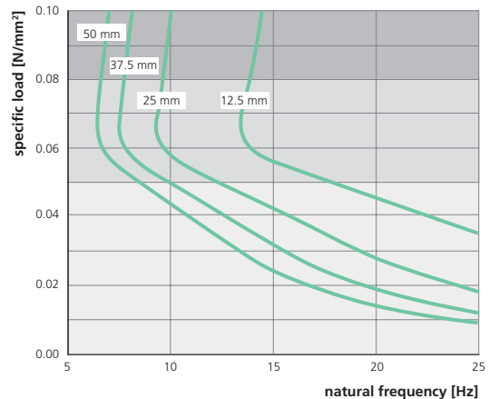
natural frequency shape factor: q=3
