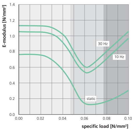
modulus of elasticity shape factor: q=1.5
