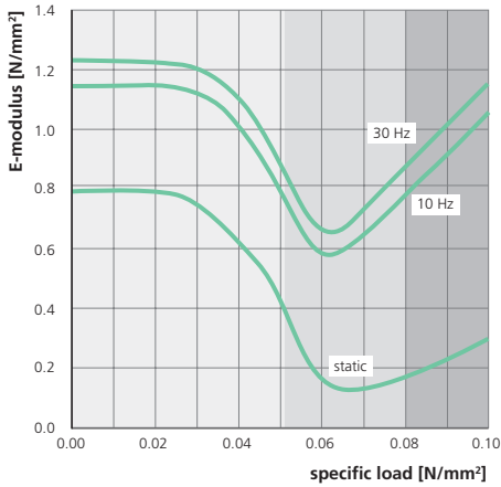
modulus of elasticity shape factor: q=6
