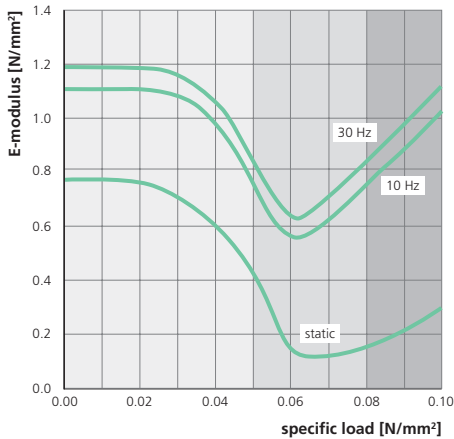
modulus of elasticity shape factor: q=3
