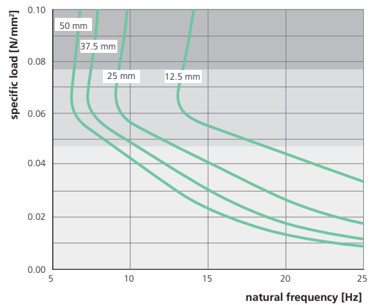
natural frequency shape factor: q=1.5
