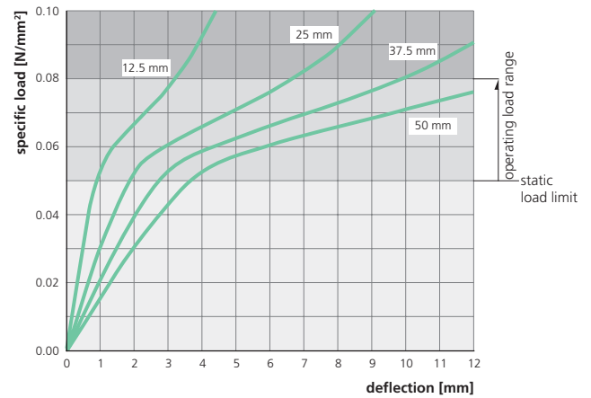
strip bearing
