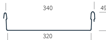
Figure 1: Profile Dimensions (nominal)
