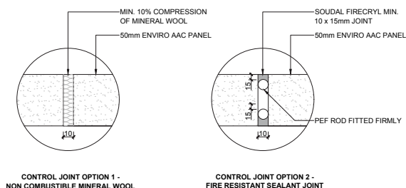
CONTROL JOINT OPTION 1 - NON COMBUSTIBLE MINERAL WOOL
