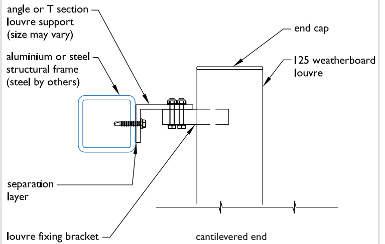
PLAN - BRACKET FIXED 125 WEATHERBOARD LOUVRE
