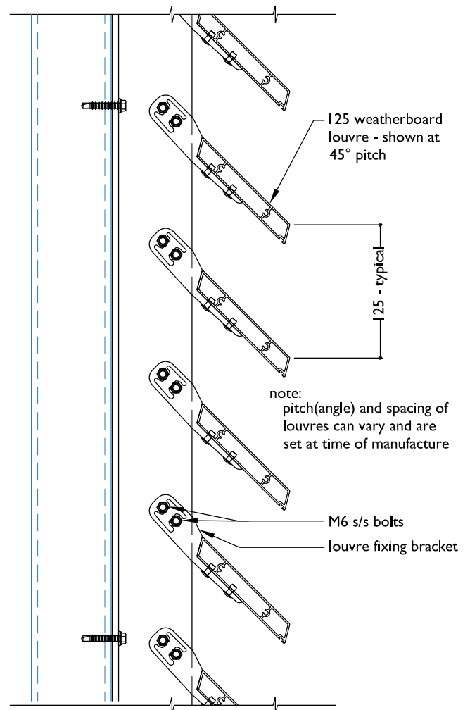
SECTION - BRACKET FIXED 125 WEATHERBOARD LOUVRE
