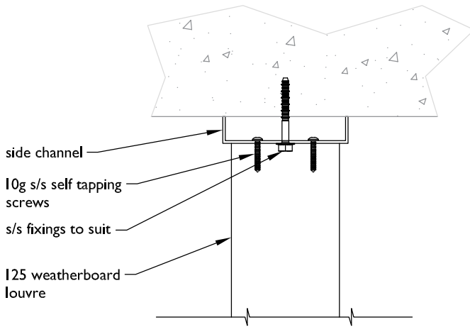
SECTION - END FIXED 125 WEATHERBOARD LOUVRE
