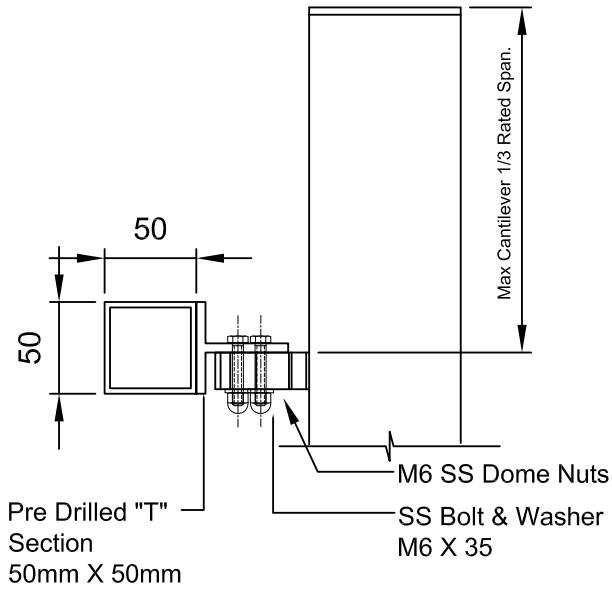
TYPICAL DETAIL // SHOWING CANTILEVER PLAN
