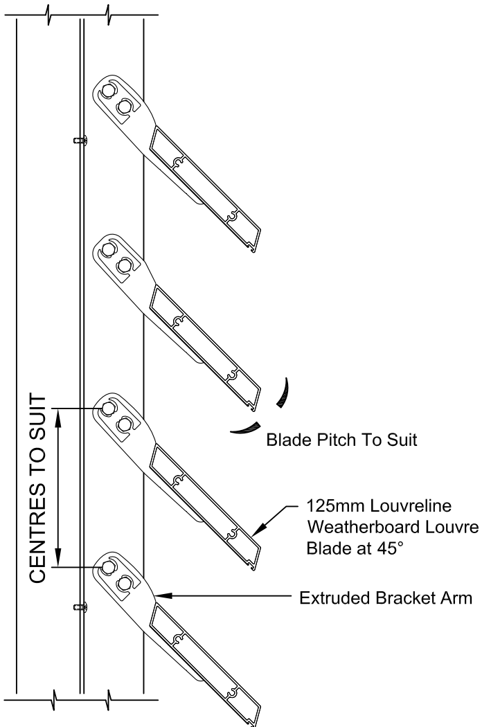
TYPICAL DETAIL // SHOWING CANTILEVER END ELEVATION
