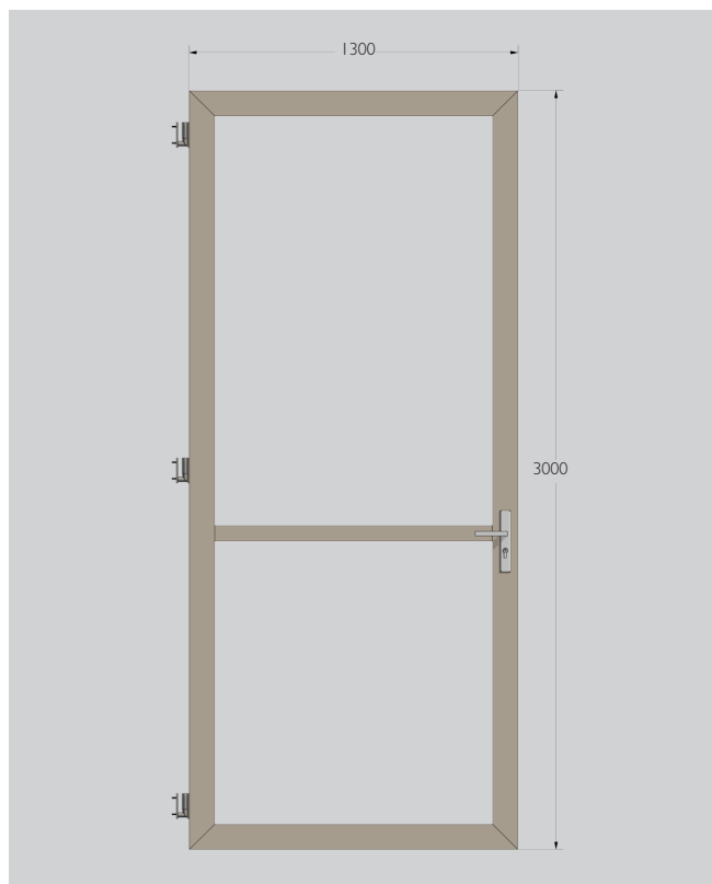
ULTRA WELDED HINGED DOOR - RECOMMENDED MAX SIZE
