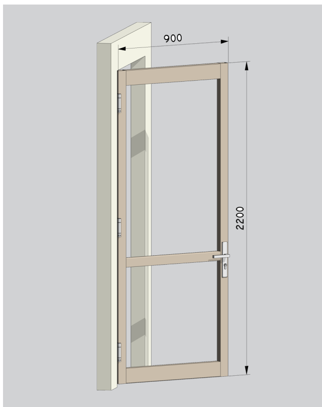
STANDARD HINGED DOOR RECOMMENDED MAX SIZES
