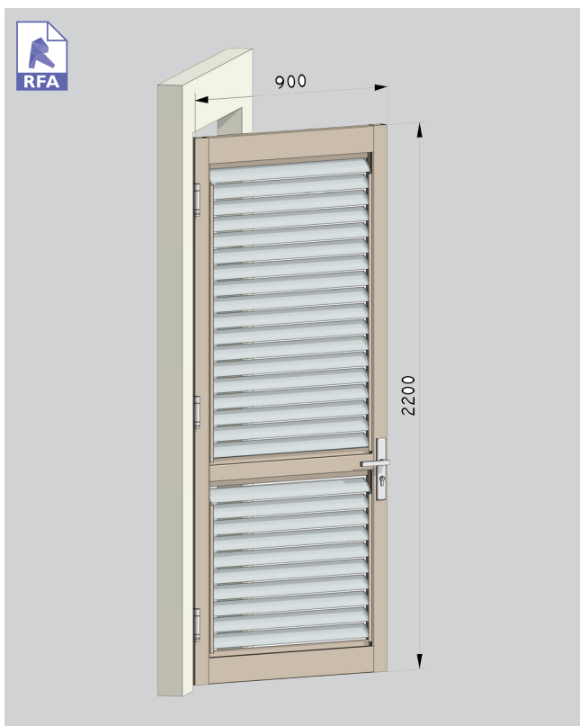
STANDARD HINGED DOOR
