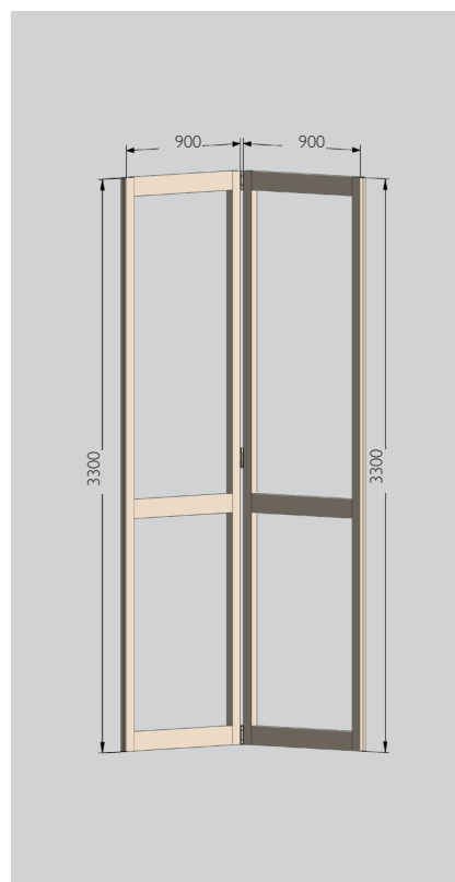
MAX PANEL SIZE 3300X900 MAX PANEL WEIGHT 100KGS
