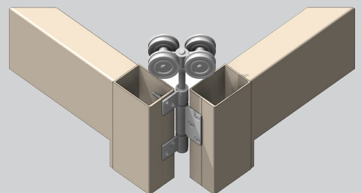
TYPICAL TOP HUNG DETAILS
