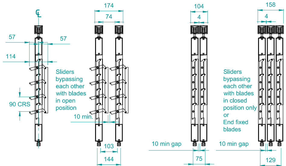
End-fixed Bellavista Heavy (dimensions) Coastal 250 Top Hung Slider
