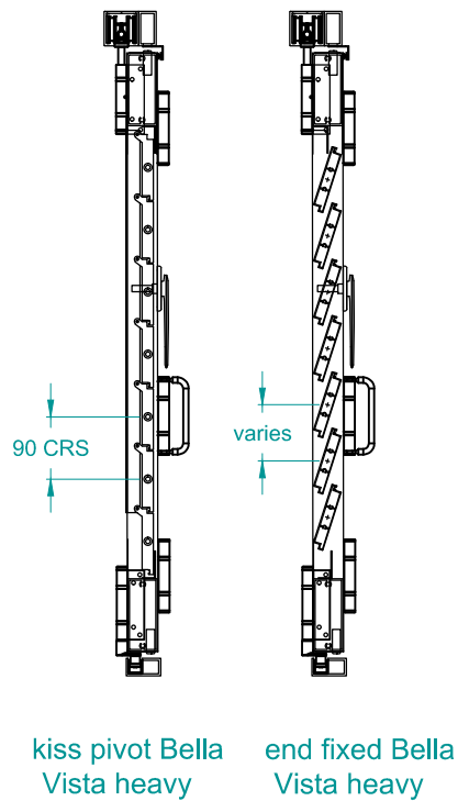
95MM BELLA VISTA HEAVY KISS PIVOT AND END FIXED
