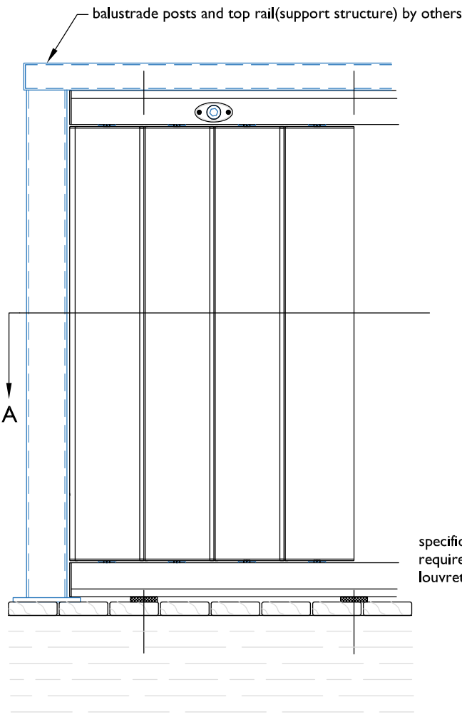
ELEVATION - I35 HI SPAN AS STANDARD BALUSTRADE INFILL
