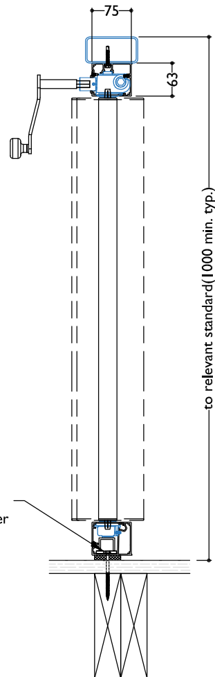
SECTION I35 HI SPAN STANDARD HEIGHT
