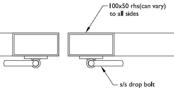
PLAN SECTION - DOUBLE PIVOT GATE JUNCTION
