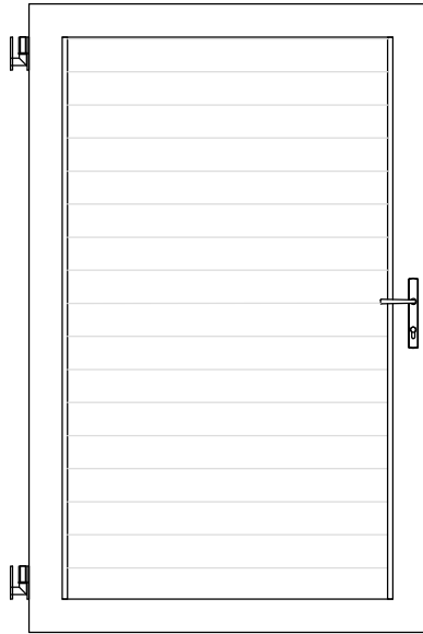
single gate (viewed from outside)
