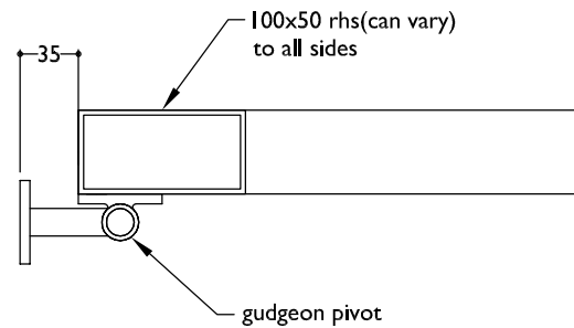
PLAN SECTION - SIDE PIVOT(ALTERNATIVE)
