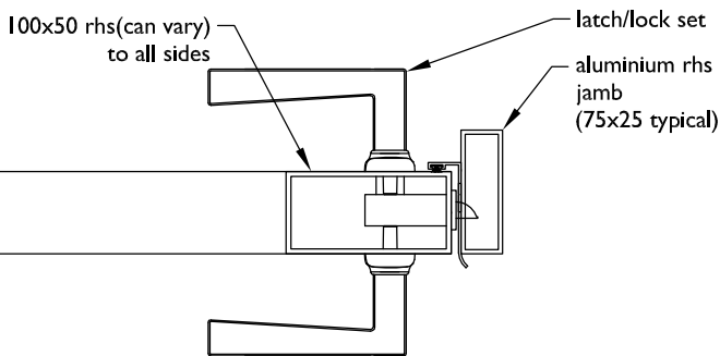
PLAN SECTION - LATCH SIDE JAMB
