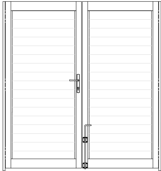
double pedestrian gate (viewed from inside)
