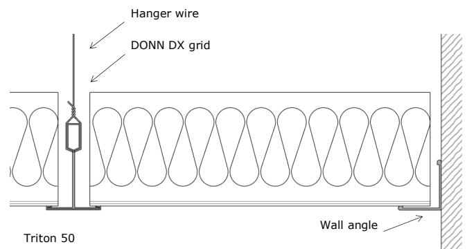
Detail: Triton 50 ceiling tiles suspended on Rondo Donn® DX Grid
