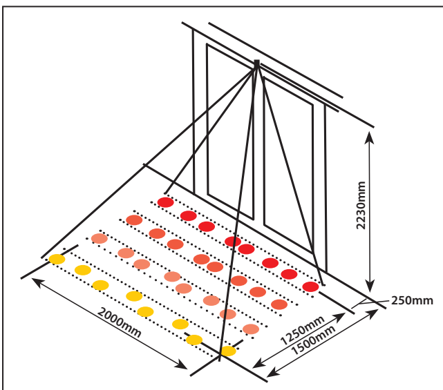
▲ Detection area of overhead sensor - fully adjustable!
