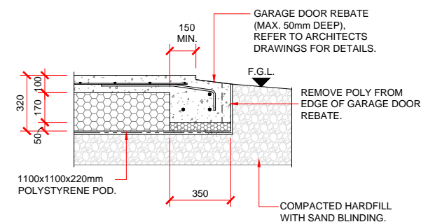
GARAGE DOOR REBATE DETAIL
