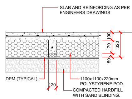
INTERNAL RIB DETAIL
