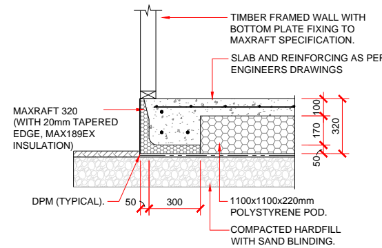
EXTERNAL FOOTING DETAIL 20mm TAPERED - 90mm/140mm FRAMING
