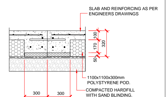
FREE JOINT / CONTROL JOINT DETAIL
