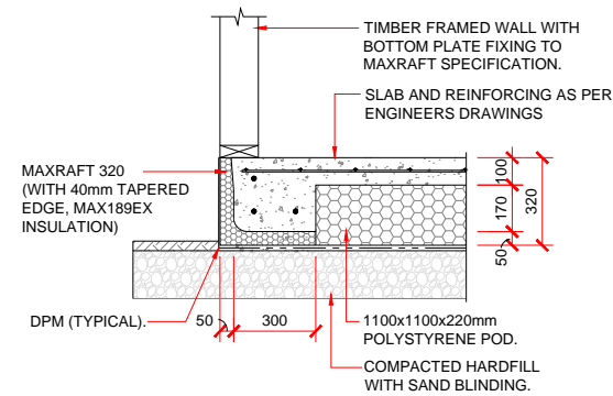
EXTERNAL FOOTING DETAIL 40mm TAPERED - 140mm FRAMING
