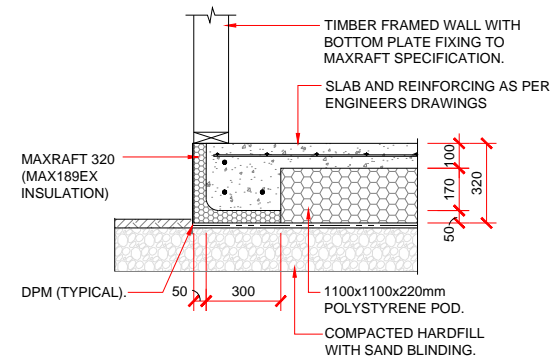
EXTERNAL FOOTING DETAIL 50mm STRAIGHT - 140mm FRAMING
