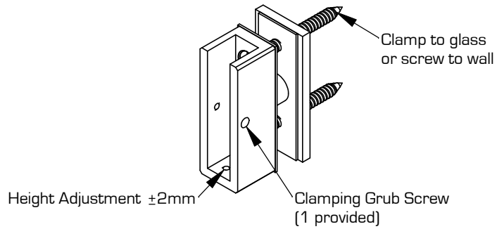
Wall mount assembly (cap removed)
