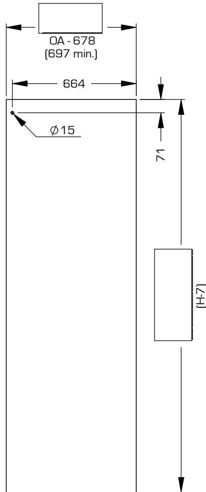
Fixed Panel 10mm Glass
