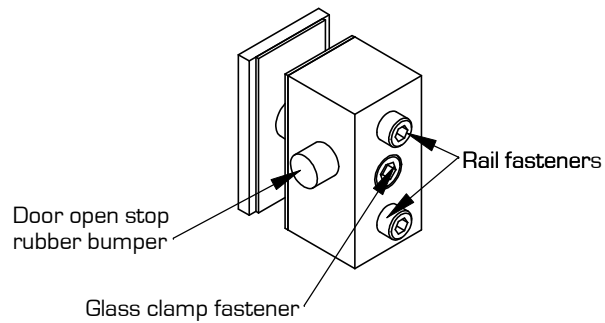
Stop/ Mount Assembly
