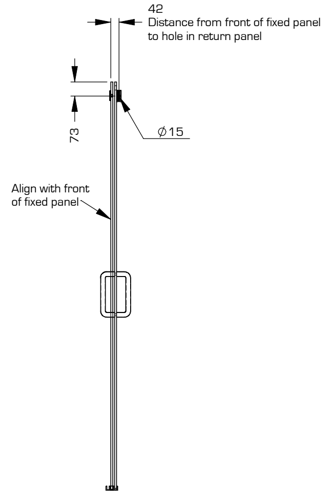
Return panel mounting detail (for rails mounted to glass)
