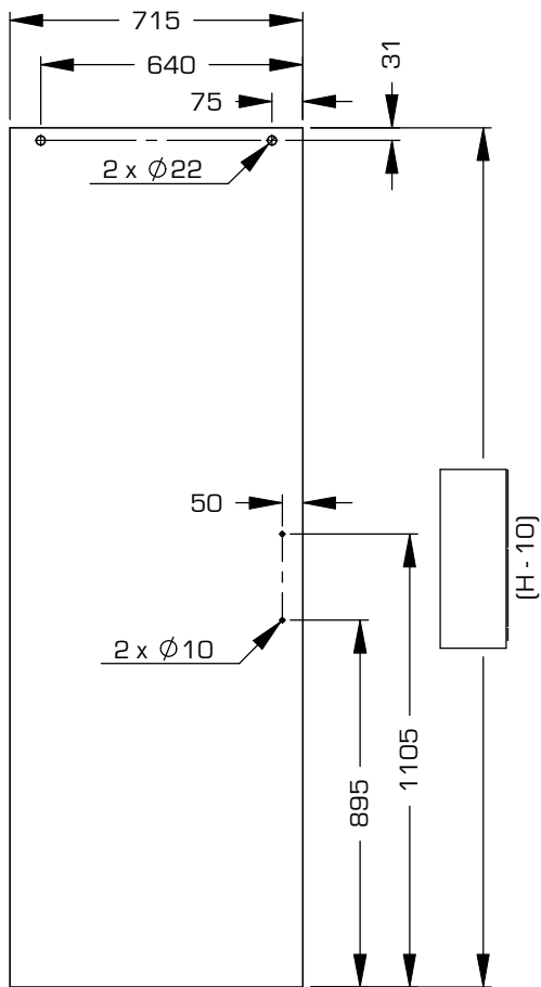
Door 10mm Glass
