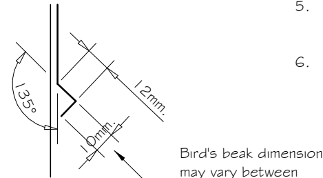
BIRD'S BEAK at bottom edge of vertical flashing
