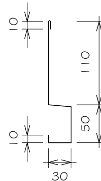
FLASHING OPTION 02
