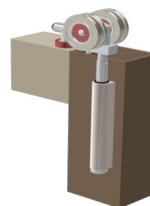
ALUMINIUM ROLLER CARRIAGE
