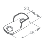
Closet Rail Bracket Part No J09
