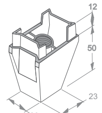
Small Foot Part No J06
