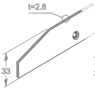
Shelf Support Part No J03
