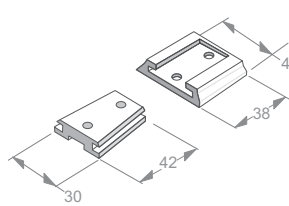
Base Cover Part No J304
