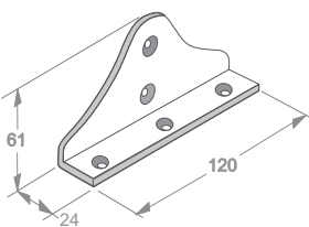
Base Part No J303
