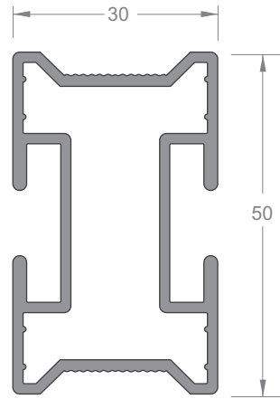
ORGANISER POLE Part No L229
