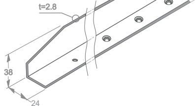
Glass Shelf Support Part No J03A
